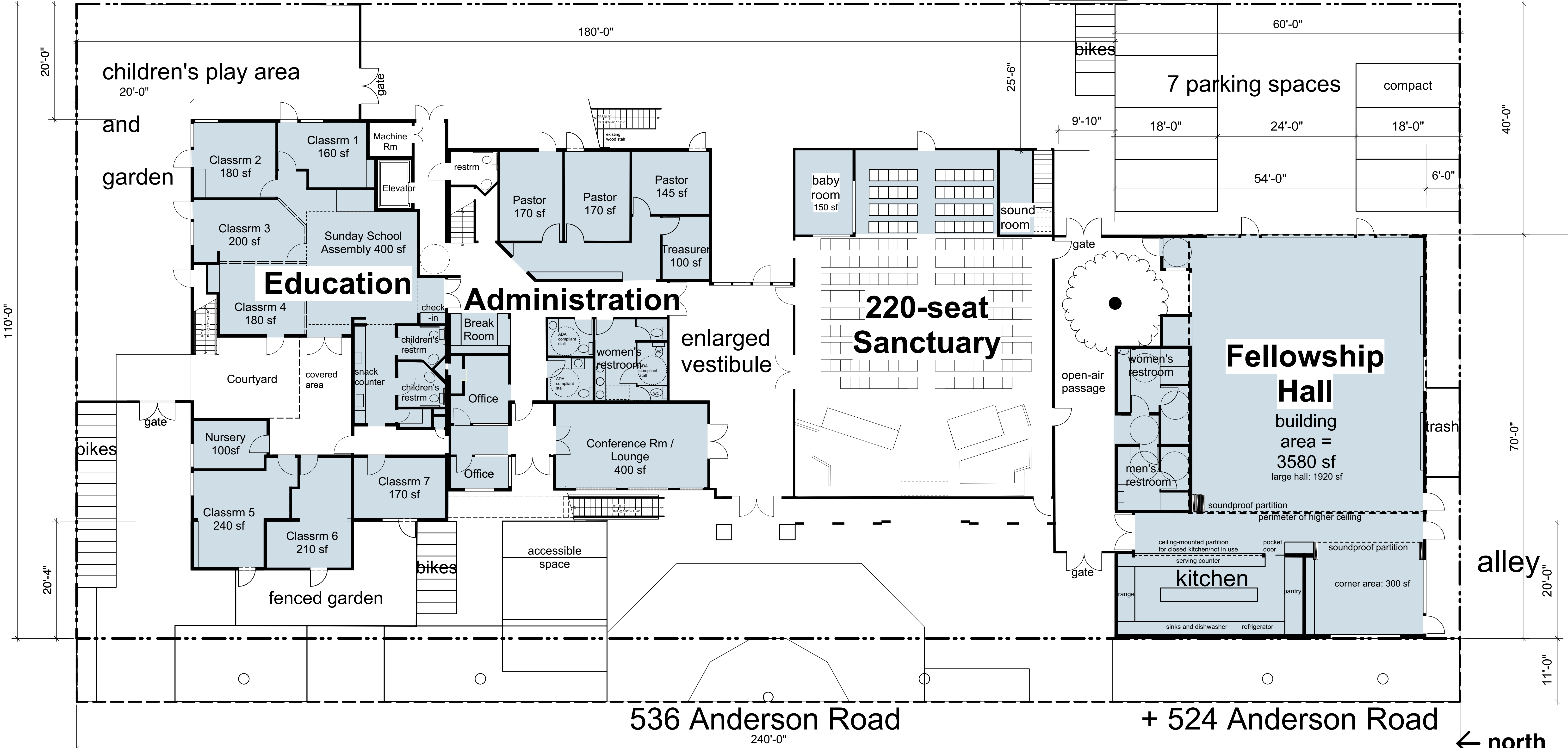
Preliminary Drawing - proposed floor plan
